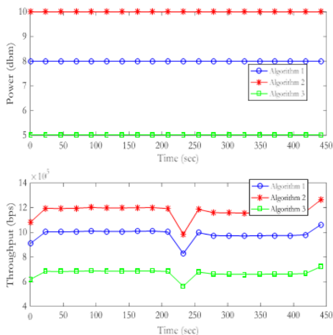
Figure 8: Femto power and throughput graphs for femto cell one (10 in topology diagram)
