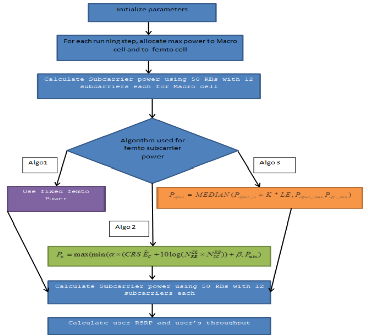
Figure 3: Flowchart for Femto power calculation and throughput calculation
